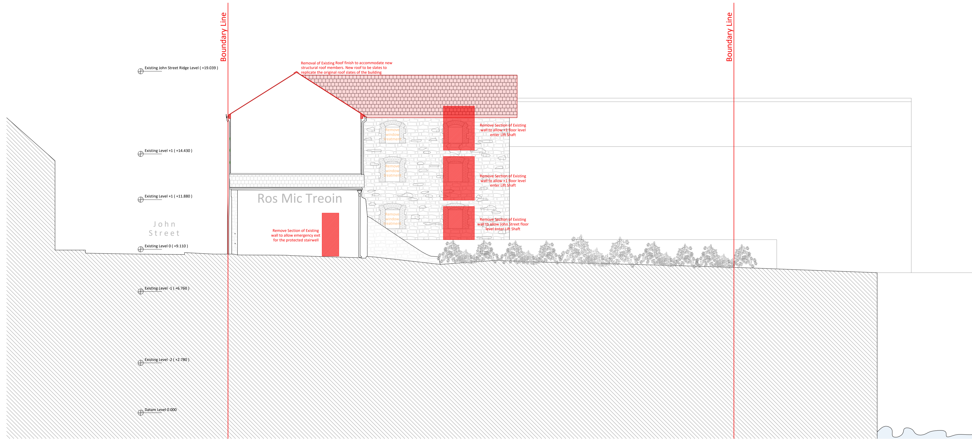
02 North (Carpark) Demolition Elevation As Existing Scale: 1:100
